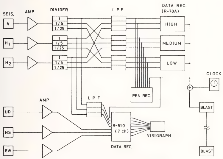
Fig. 2 Block diagram of the observation system.
